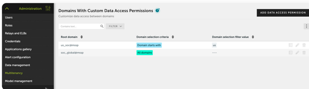
Users have the ability to provision and configure data access for multiple tenants using self-service capabilities.
