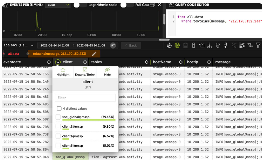
Global search capabilities help security teams hunt for IOCs across multiple tenants.
